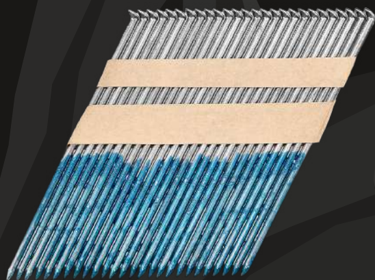
34° D-head nails 4.6x160mm
