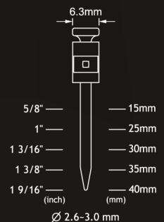
Ballistic Shank
