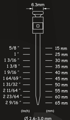
Ballistic Shank
