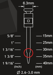
Stepped Shank
