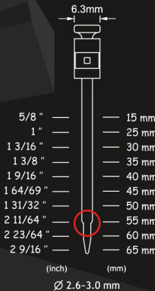
Stepped Shank
