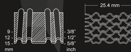
CF254S
